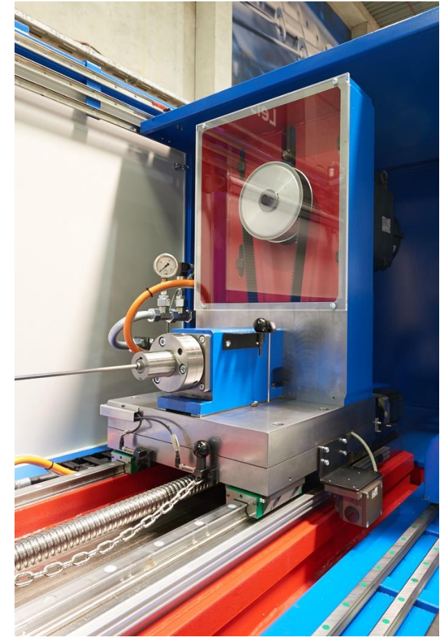
Drill spindle unit
